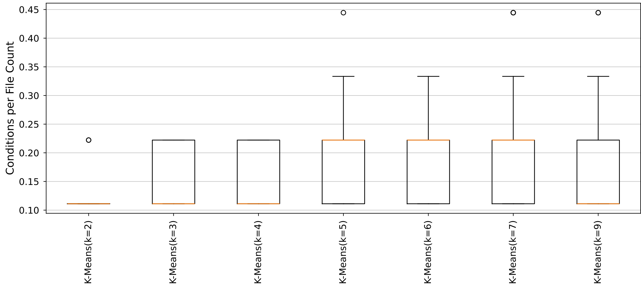
YARA Rules Conditions per File Count Distribution (Cluster11_Size9 dataset)
